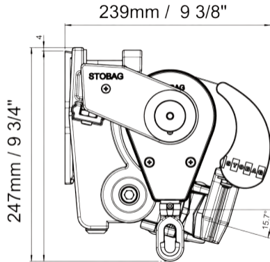
Wall mount
